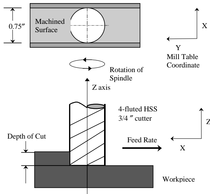
Figure 3. Experimental setting of the work piece and the end mill process
