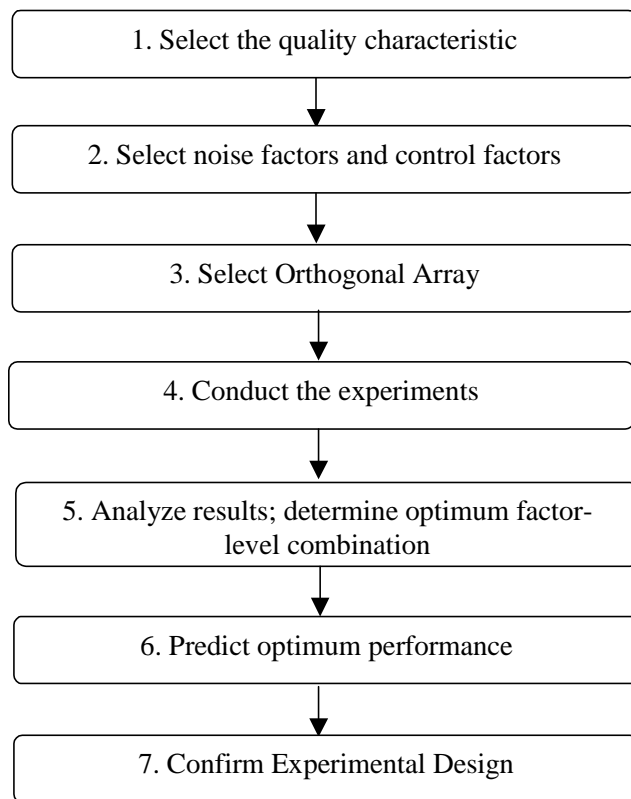
Figure 2. Procedure and steps of Taguchi parameter design
