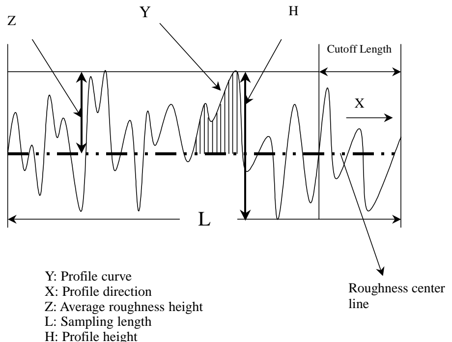
Figure 1. Surface roughness profile.
