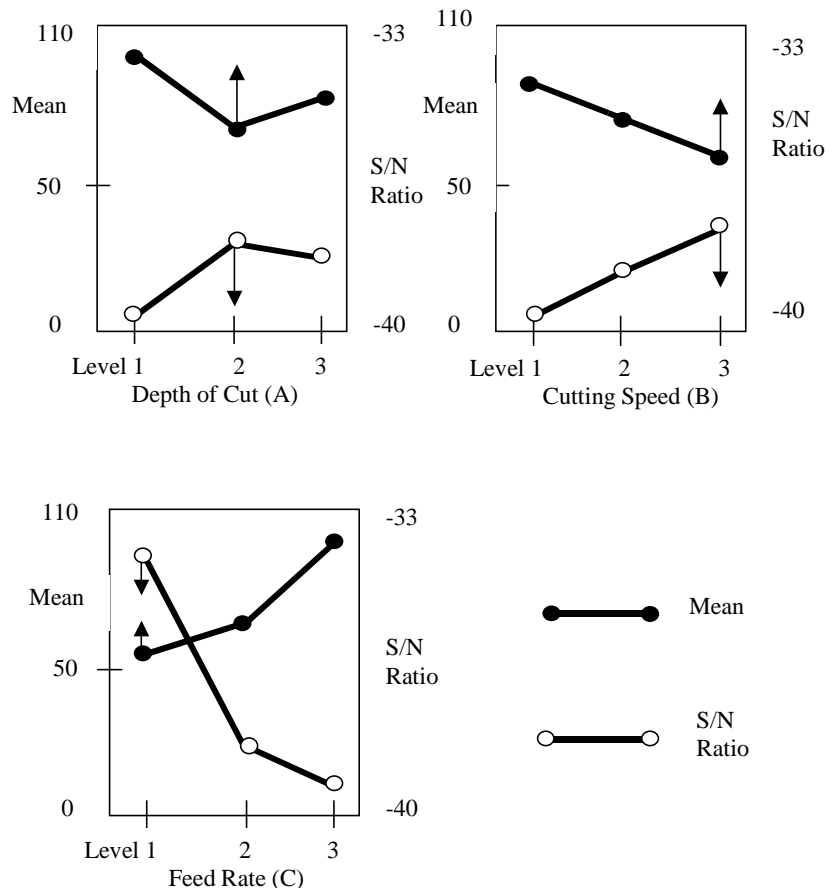
Figure 4. Response graphs of three significant cutting factors (↑ indicates the optimal level of response mean; ↓ indicates the optimal level of S/N ratio)
