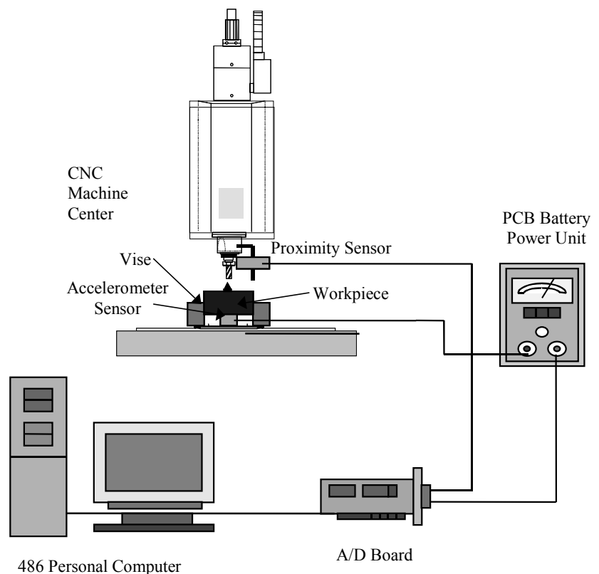
Figure 1. Experimental Setup
