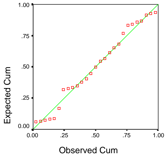
Figure 4. Normal P-P Plot of Regression Standardized Residual Dependent Variable: Vibration Vi
