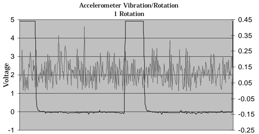
Figure 2. Vibration data from 1 trial run. One-inch diameter tool at 20 ipm Feed rate.
