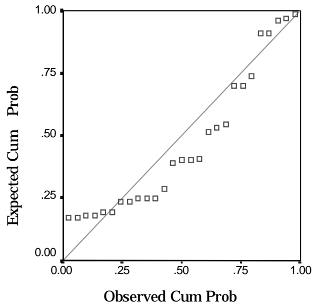
Figure 3. Normal P-P Plot of Regression Standardized Residual Dependent Variable: Profilometer Ra
