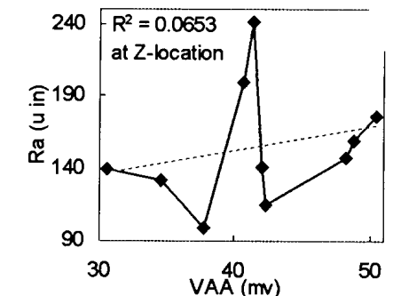
Figure 5. The relationship between the surface roughness (Ra) and the vibration amplitude average (VAA) at different locations.
