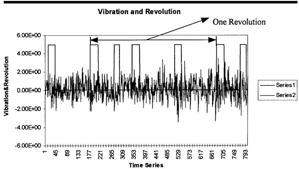
Figure 3. Original X Vibration under feed rate 2 ipm
