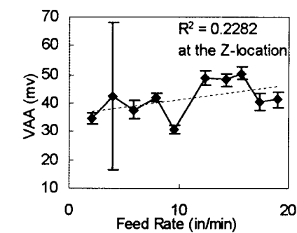
Figure 4. The relationship between the vibration amplitude average (VAA) and the feed rates at different sensor locations.
